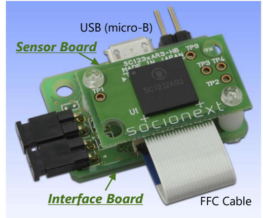
Evaluation Kit of SC1232AR3
