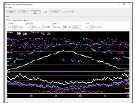
Plot of distance (Upper white-line) * Vertical-axis: Distance from sensor, Horizontal-axis: Time
