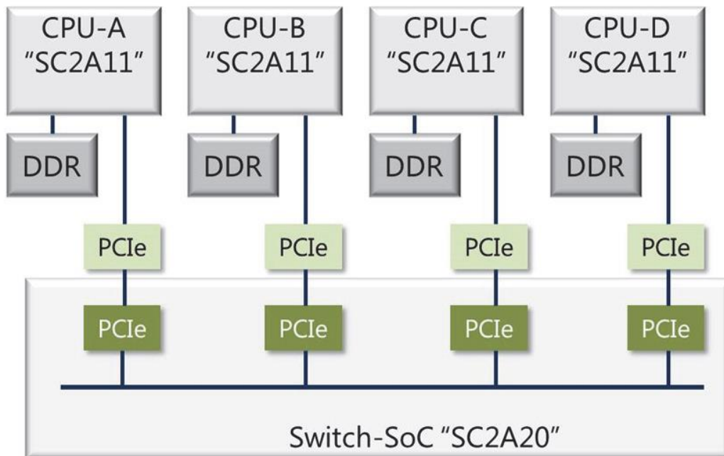
Figure 1: CPU Connection by SC2A20
